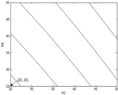
Figure 9. Monotonic surface representing bottle weight,
