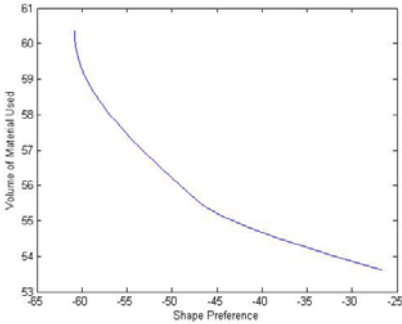
Figure 10. Pareto frontier for multiobjective optimization.
