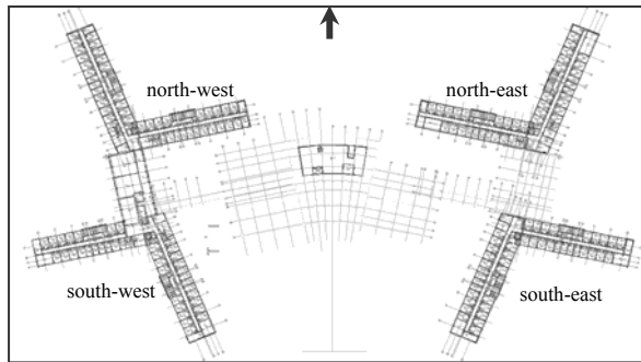
Figure 1: The plan of Bursley dormitory showing the four different wings
