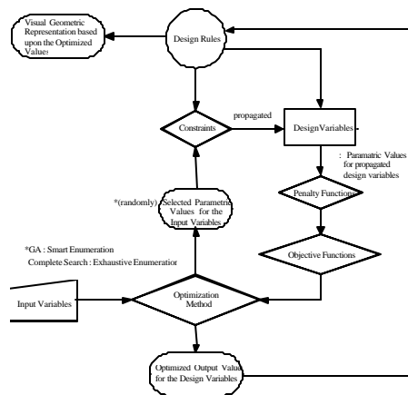
Figure 4 The structure of the synthesis component of Hermes
