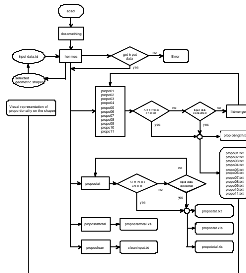
Figure 3 The structure of the analysis component of Hermes
