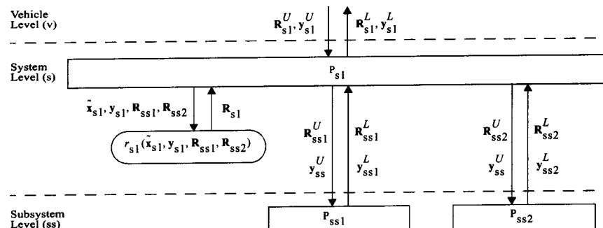
Fig. 2 Flows from/into the system-level design problem
